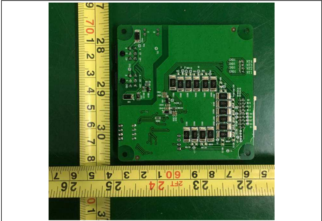
PCB general viwe -1 of battery expansion modules
