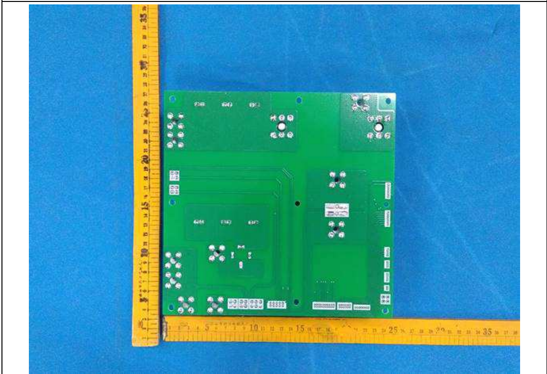
PCB general view -2 of main power board
