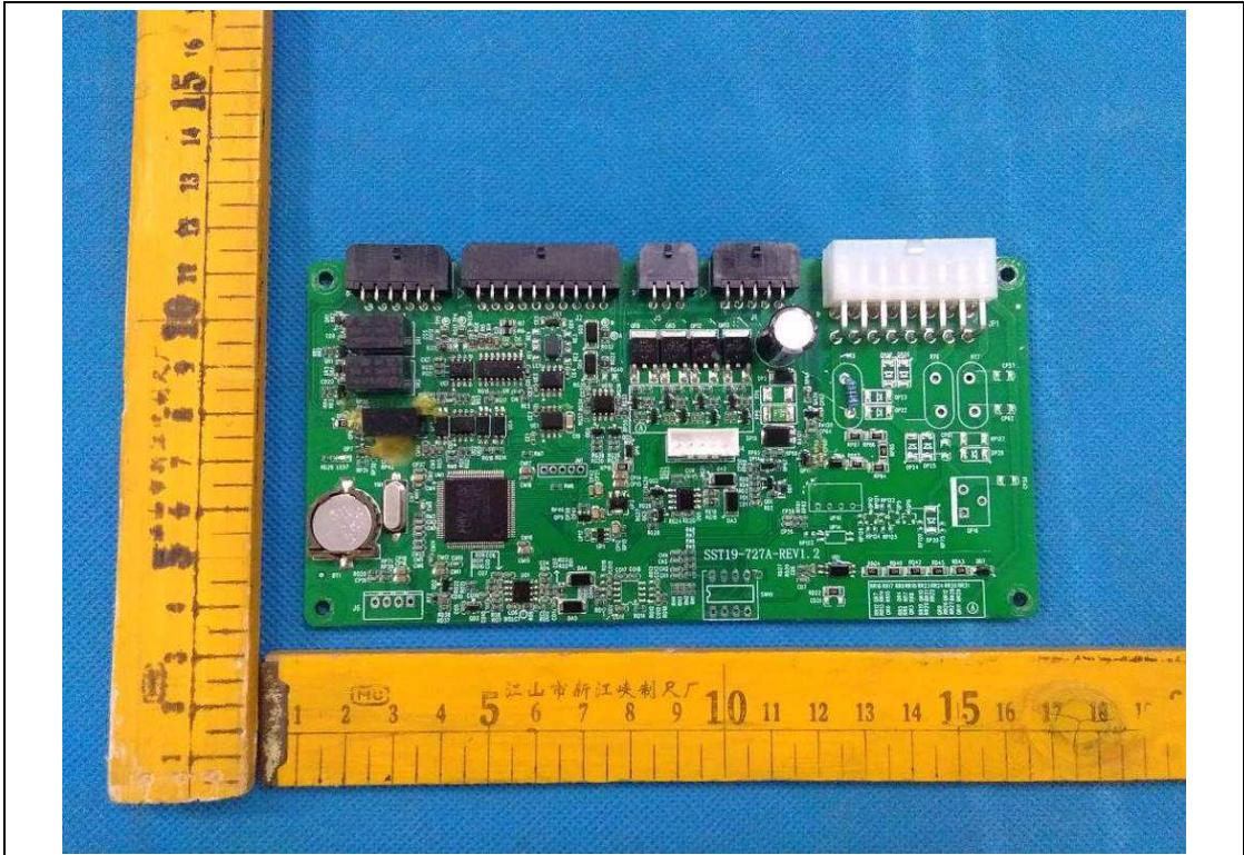
PCB general view -1 of BMS control board
