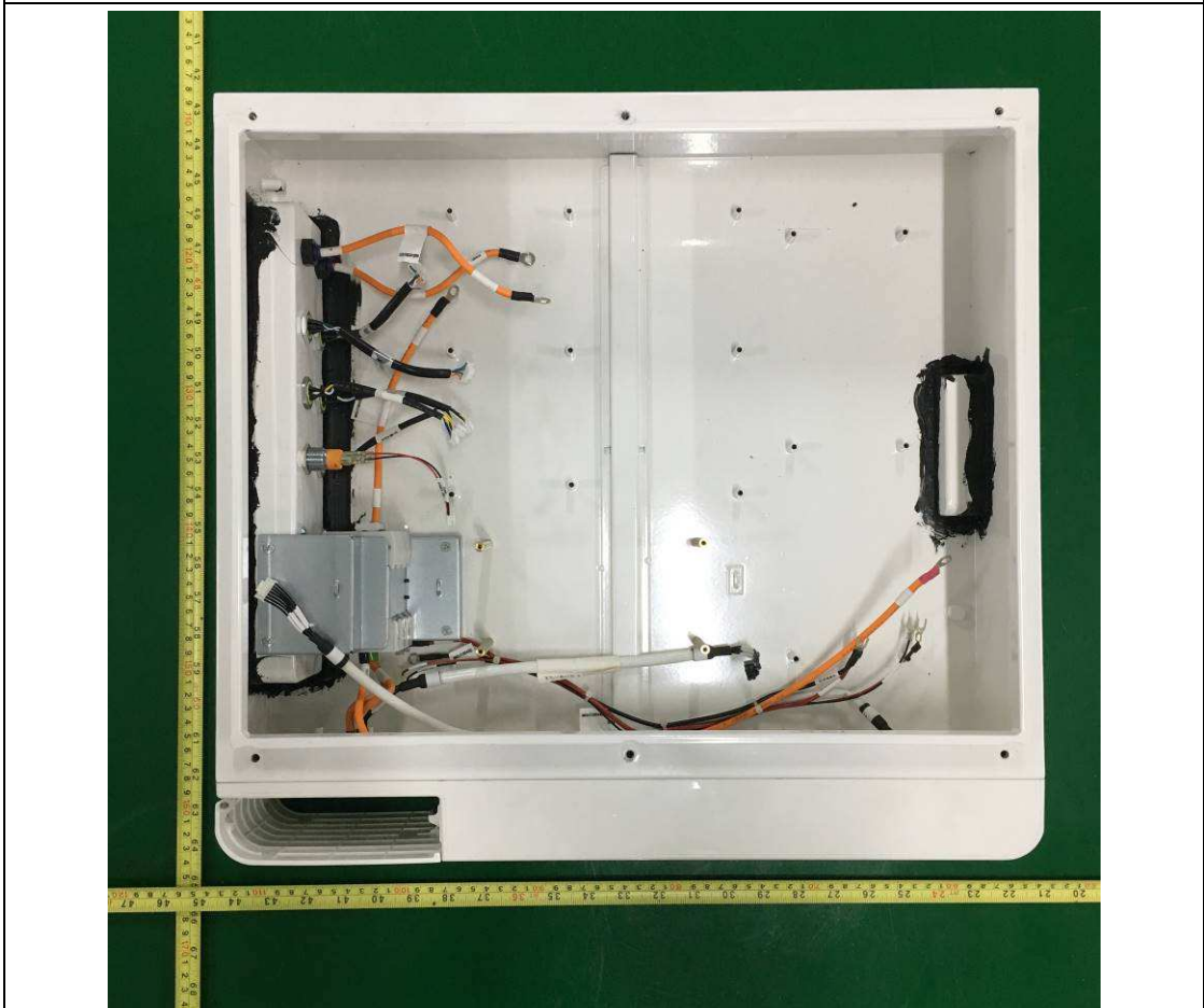
Internal view-2 of power contro module
