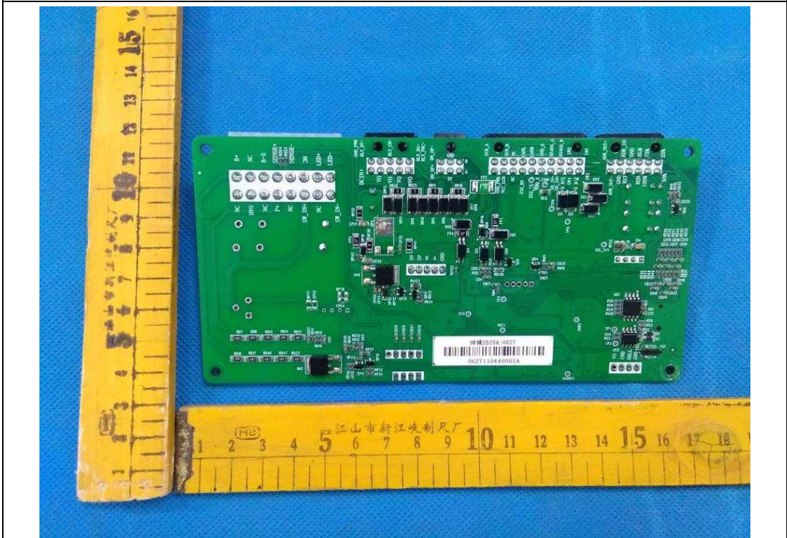
PCB general view -2 of BMS control board
