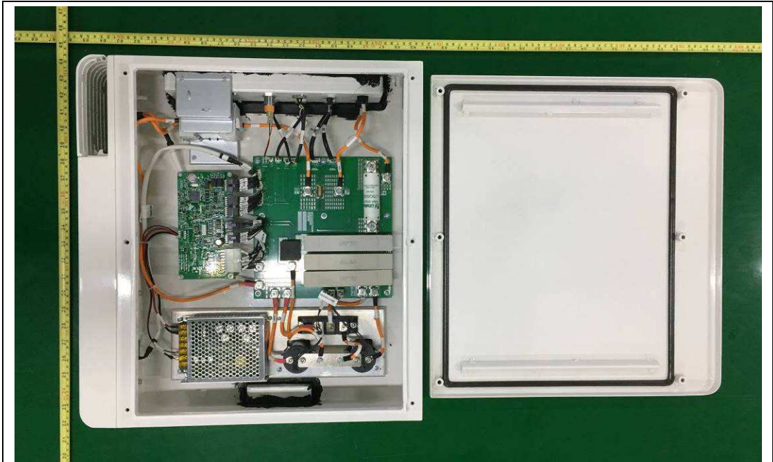
Internal view-1 of power contro module
