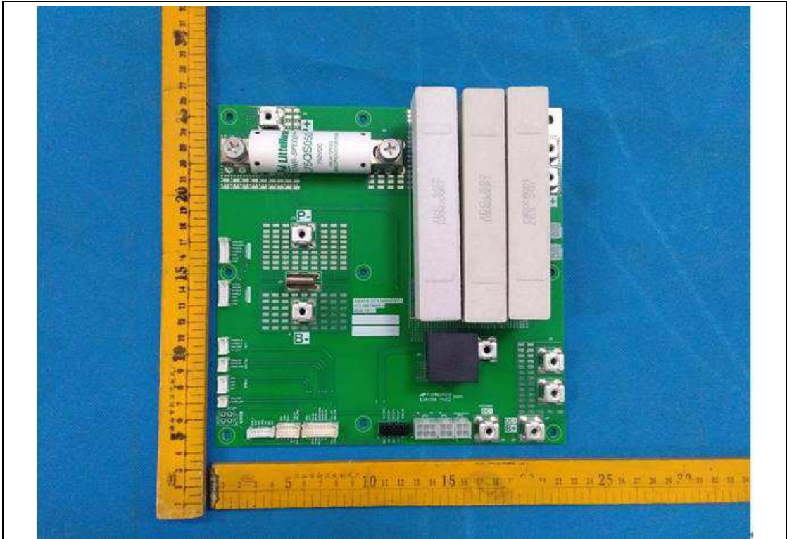
PCB general view -1 of main power board
